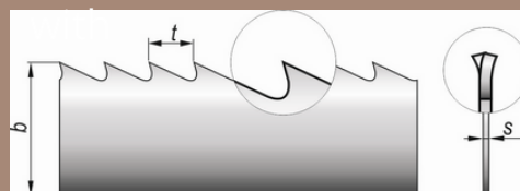
standard tooth (S)
